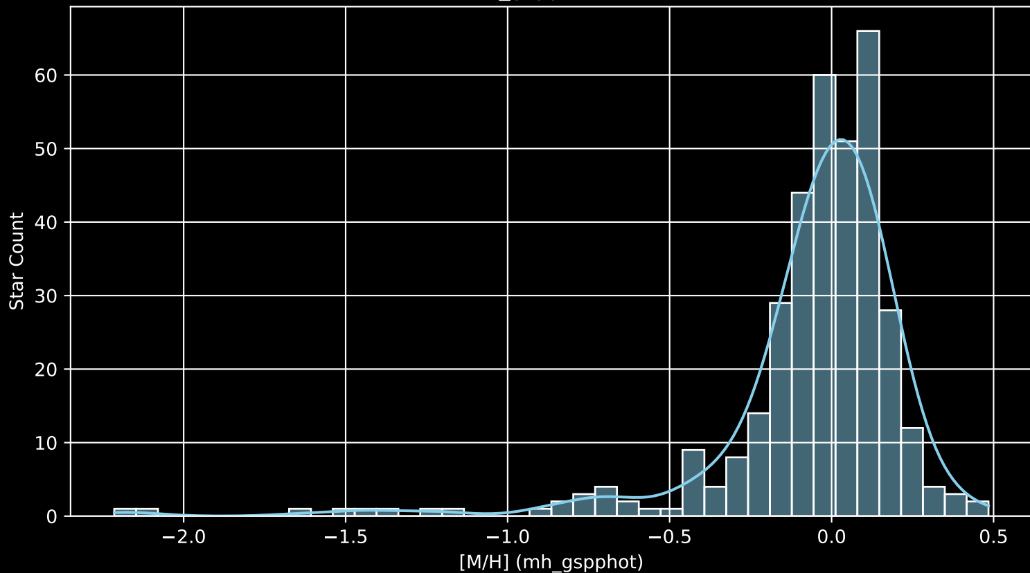
APOGEE DR17 Field: [326-06 [M/H] (mh_gspphot) (n= 356)
