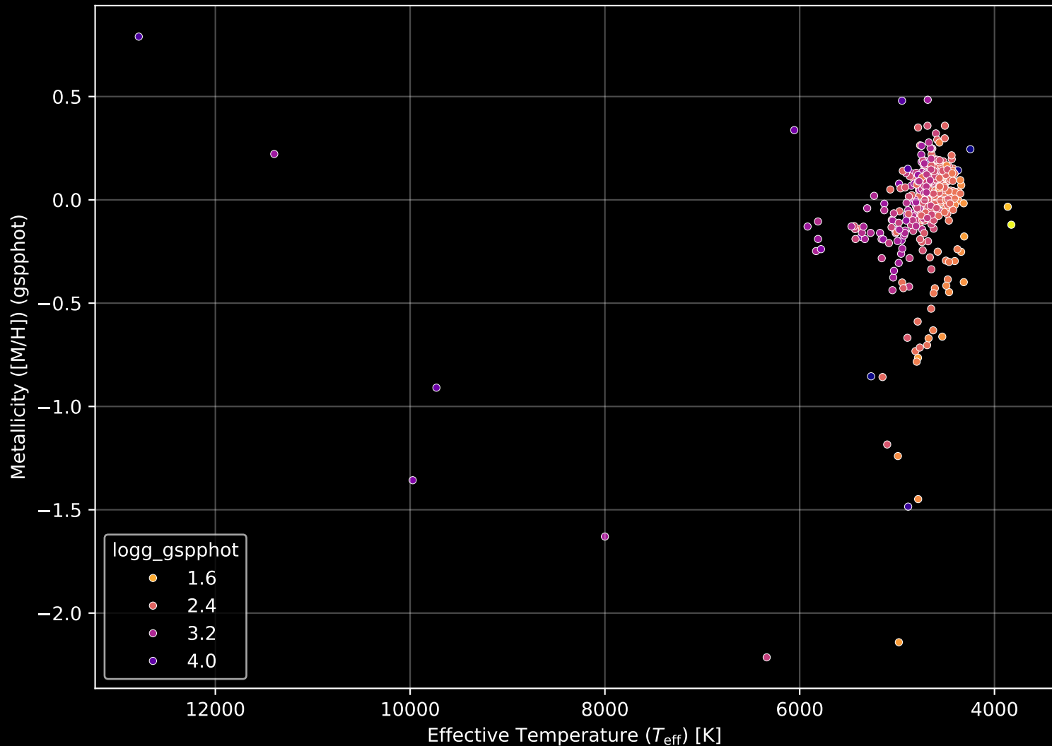
APOGEE DR17 Field: [326-06] Stellar Population Parameters (n= 357)
