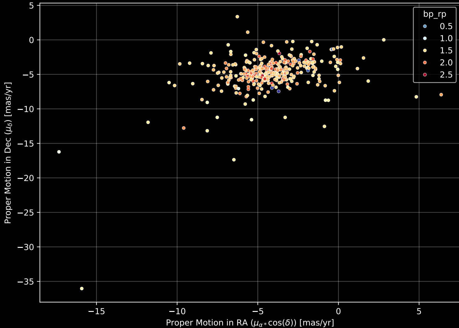
APOGEE DR17 Field: [326-06] Proper Motion Diagram (n= 357)
