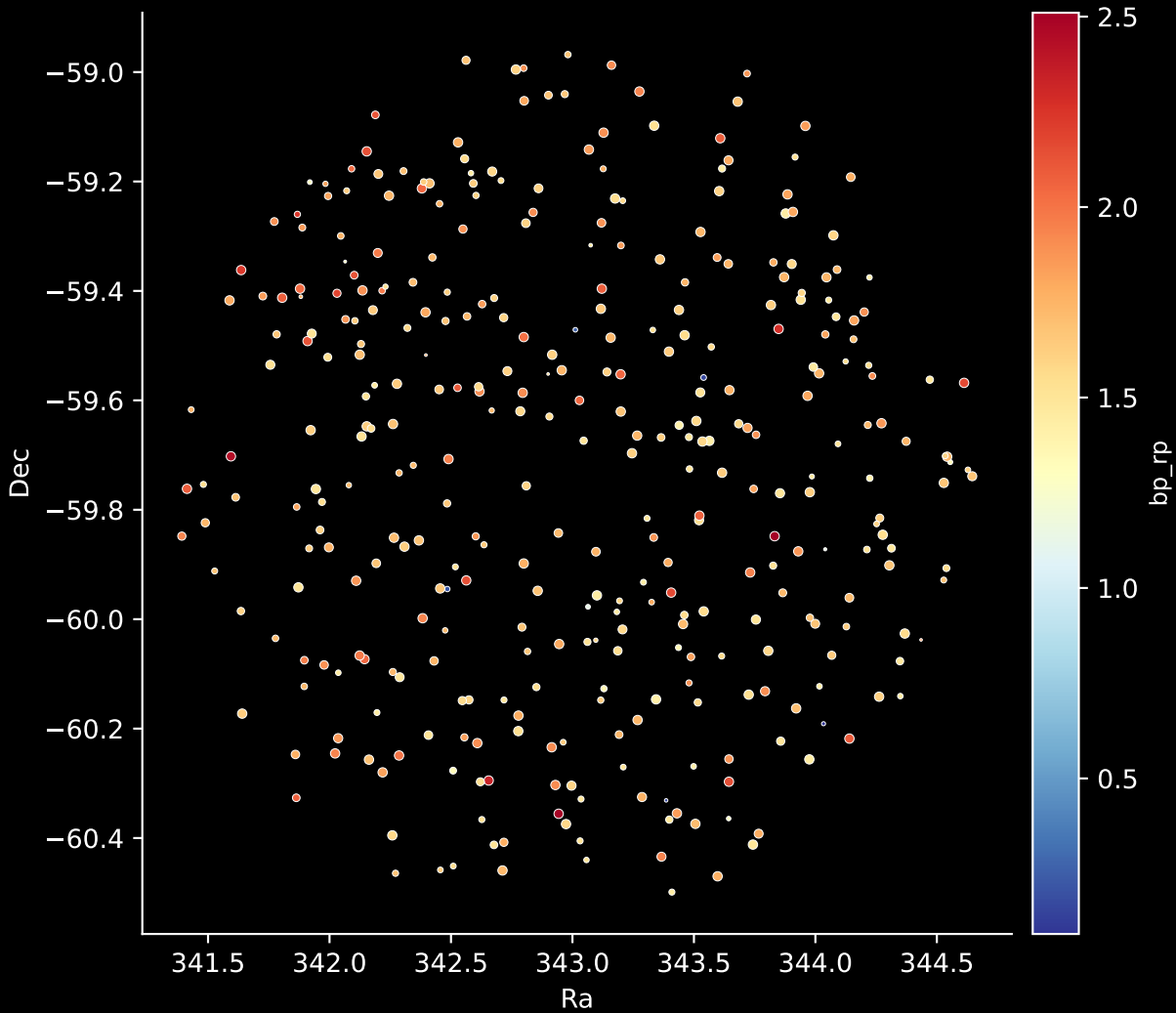
APOGEE DR17 Field: [326-06] Stars: 357
