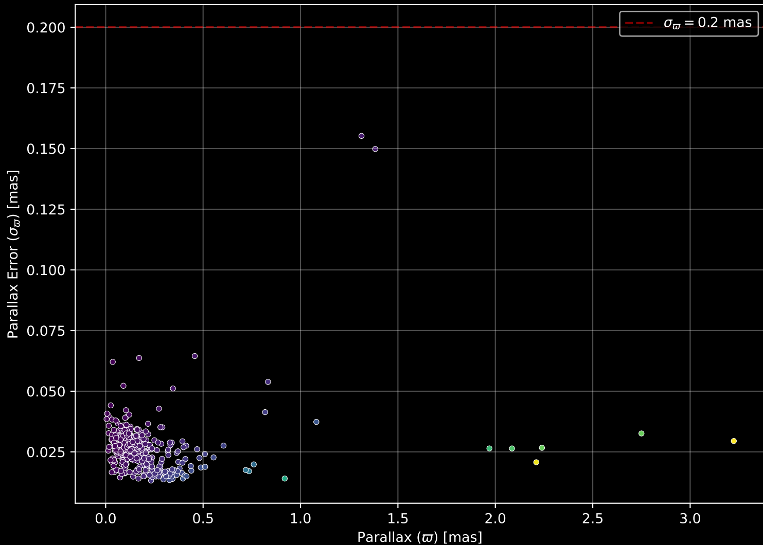
APOGEE DR17 Field: [326-06] Parallax Quality (n= 357)
