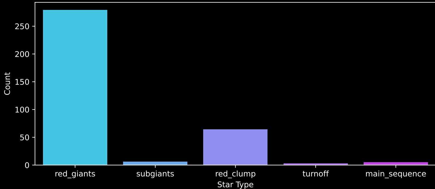
APOGEE DR17 Field: [326-06] Count plot of Star Type
