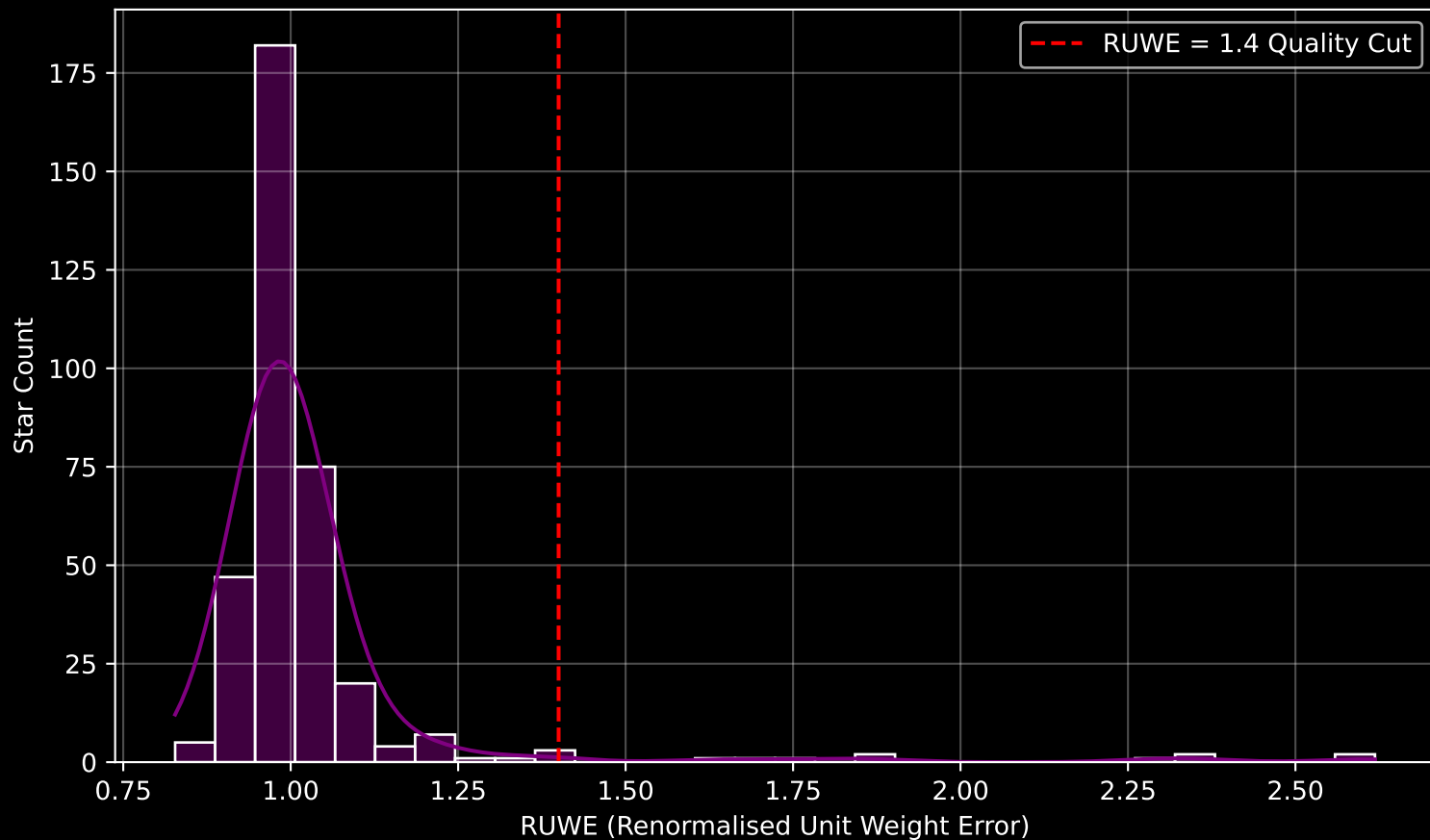
GAPOGEE DR17 Field [326-06] RUWE Distribution (n= 355)
